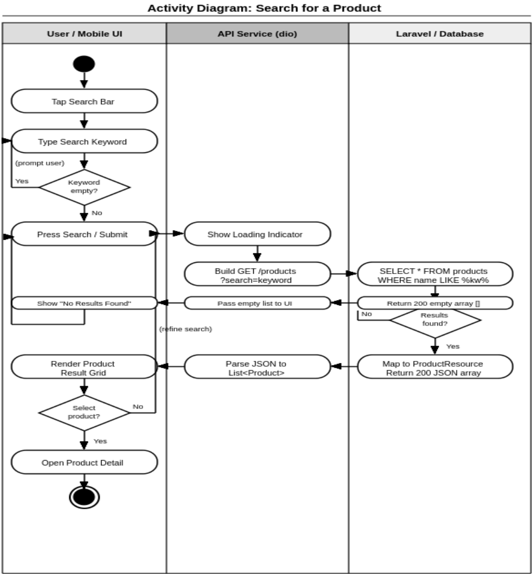
Figure 4.7 Search for a Product Activity Diagram
