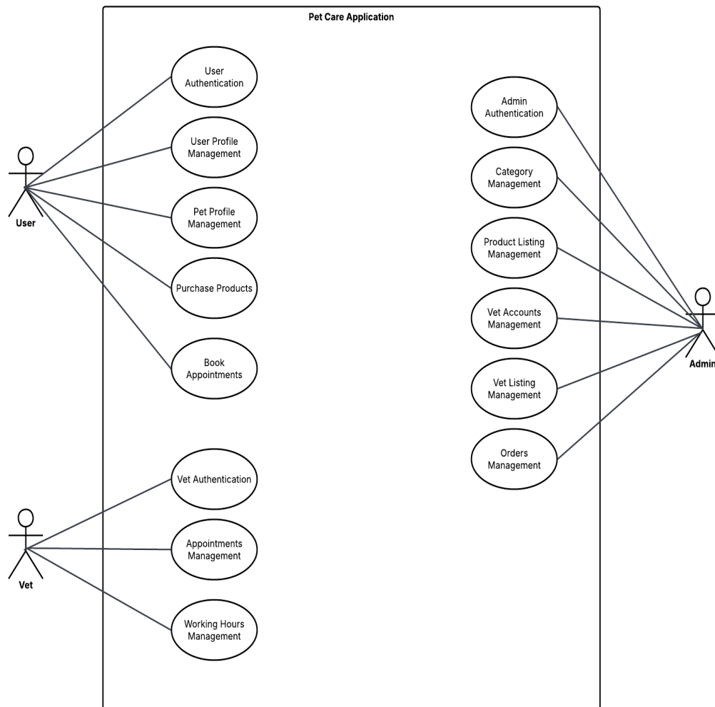
Figure 4.1 High Level Use Case Diagram
