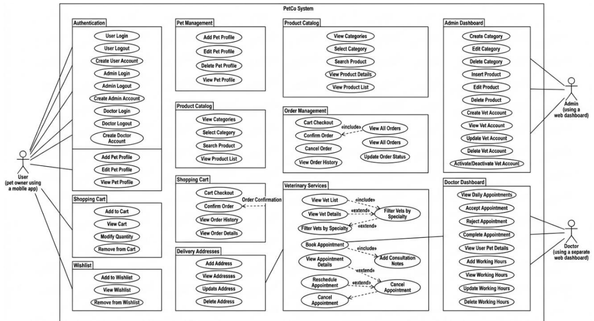
Figure 4.2 Low Level Use Case Diagram
