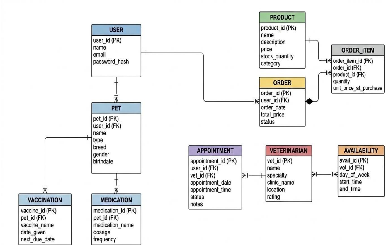
Figure 5.2 – Entity Relationship Diagram
