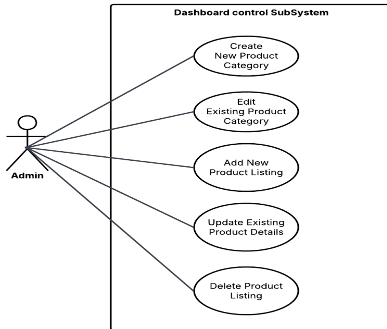
Figure 4.6 Dashboard Control Subsystem Use Case Diagram
