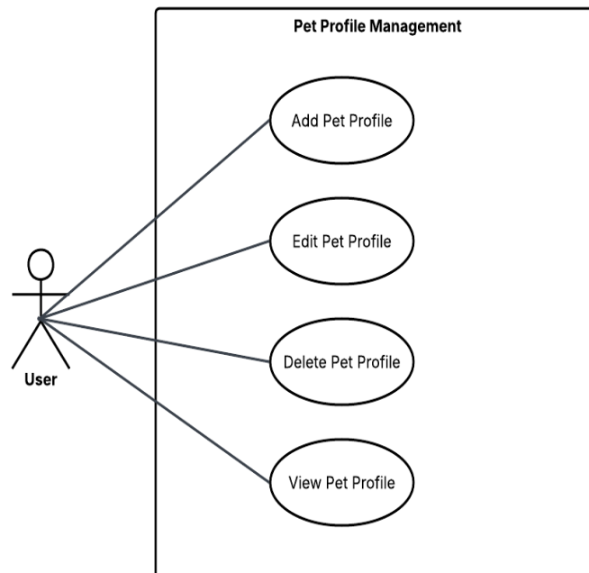
Figure 4.3 Pet Profile Management Subsystem Use Case Diagram
